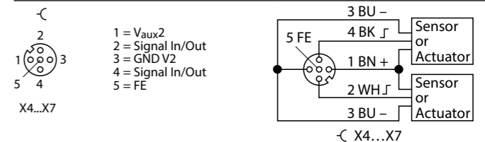
Digital channels X4...X7
