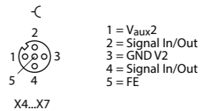
Digital channels
