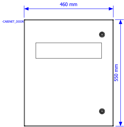
DOOR VIEW
