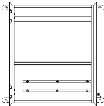
MOUNTING VIEW
